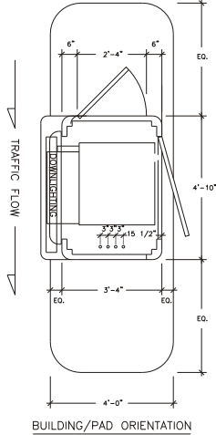
Drawing 96-007 with sign box
