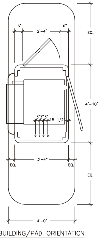
Drawing 96-007
