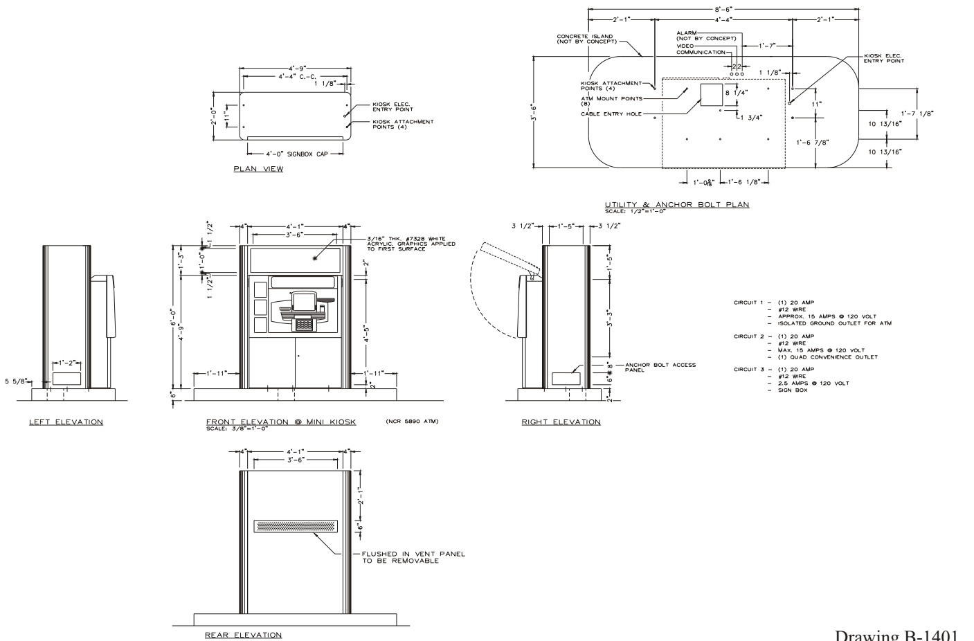
Drawing B-1401
