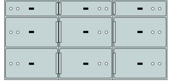
SD or SS 9 (Wt. 149 lbs.) 3 openings ea. 3" x 10" and 6 openings ea. 6" x 10"
