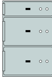
SN or ST 3 (Wt. 61 lbs.) 1 opening ea. 3" x 10", 2 openings ea. 6" x 10"
