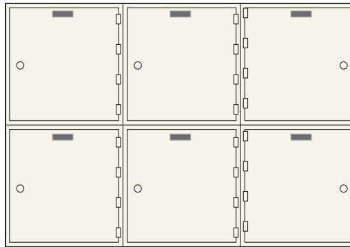
AX-6 6 openings ea. 10" x 10"
