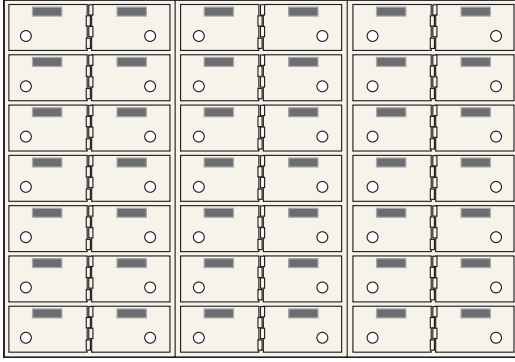
AX-42 42 openings ea. 3" x 5"
